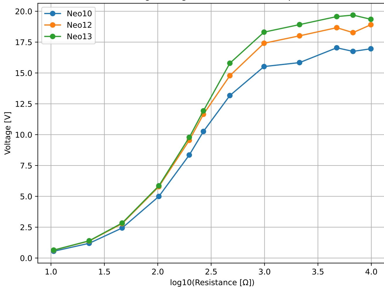
Voltage vs \log_{10}(\text{Resistance}) - 840rpm
