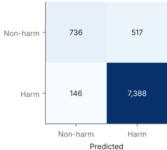
Kaggle non-IID
