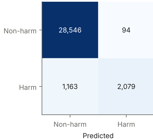
Jigsaw non-IID
