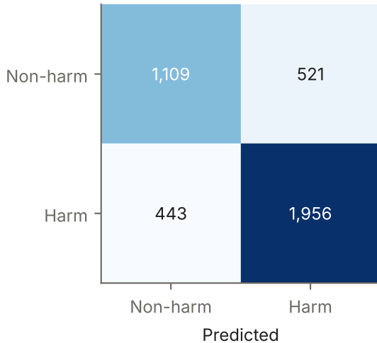
HateXplain (external)
