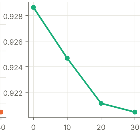
Accuracy
