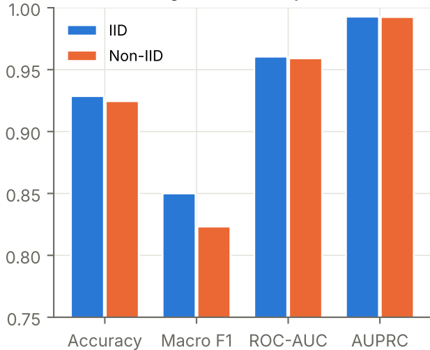
Ranking and accuracy metrics
