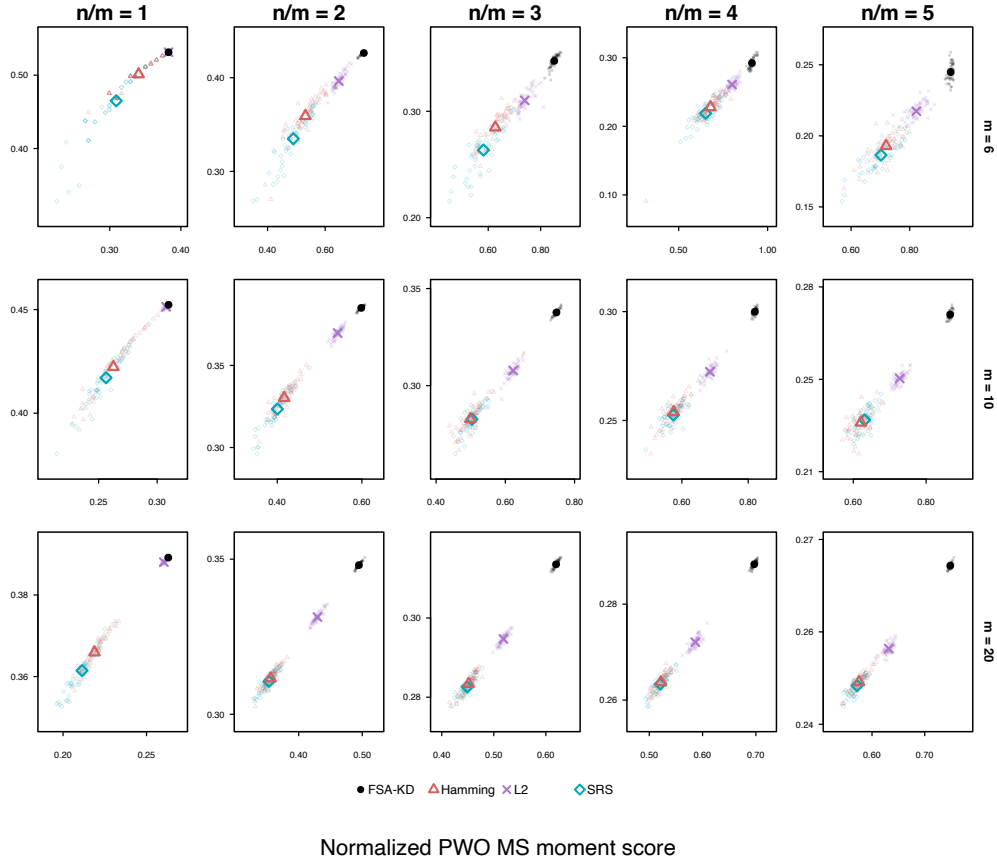
Mallows determinant-root criterion ( c = 1 )
