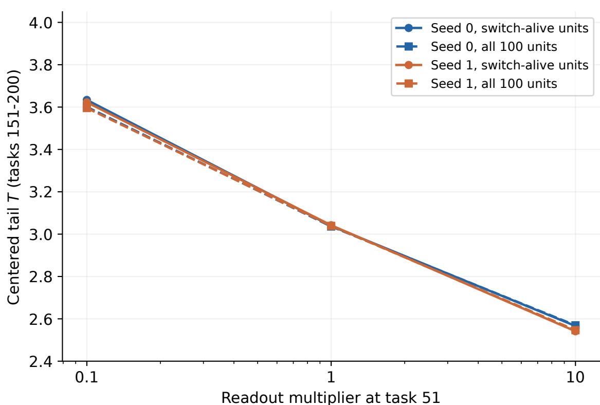
D Saved RL-MNIST: shape effect persists
