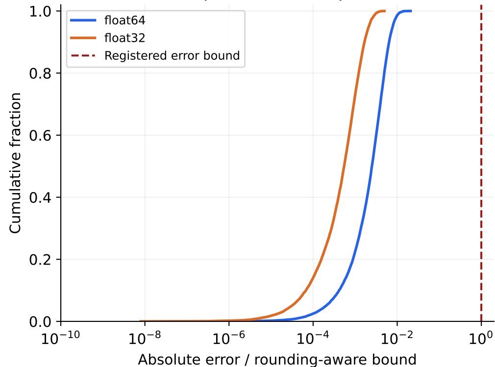
Finite-precision discrepancies
