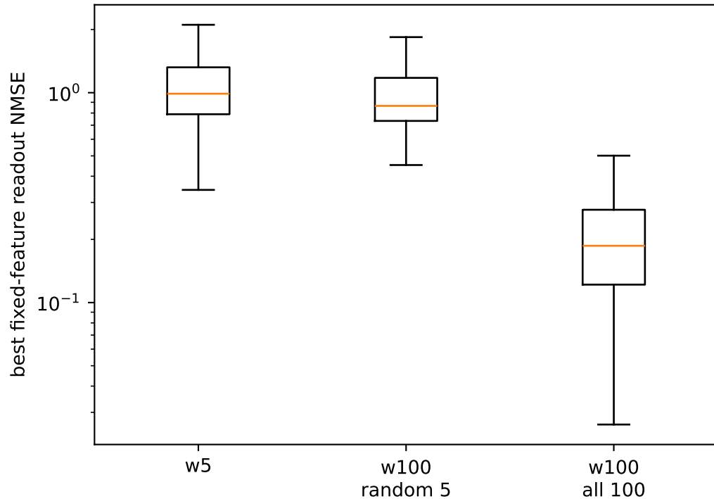
Candidate 7: exact task-support fits
