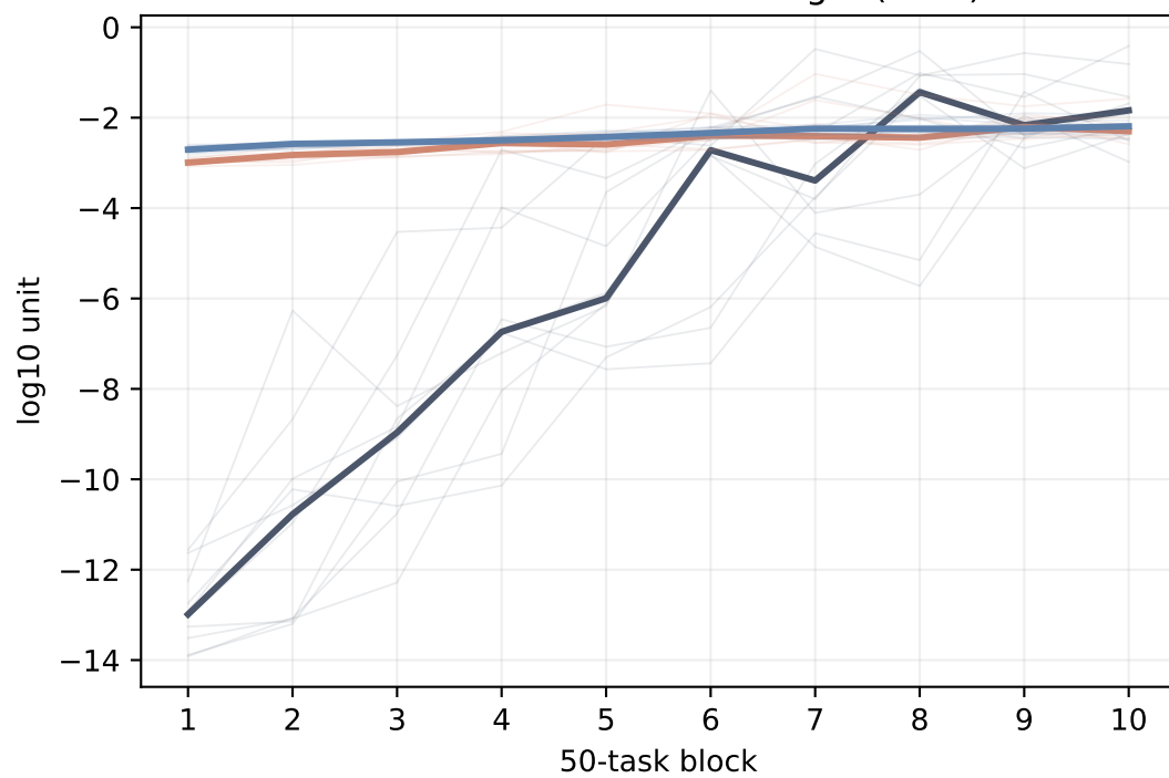
Network function: mean log10(unfit)
