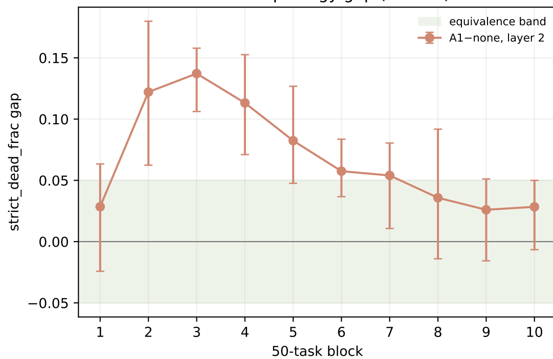
Paired morphology gap (95% CI)
