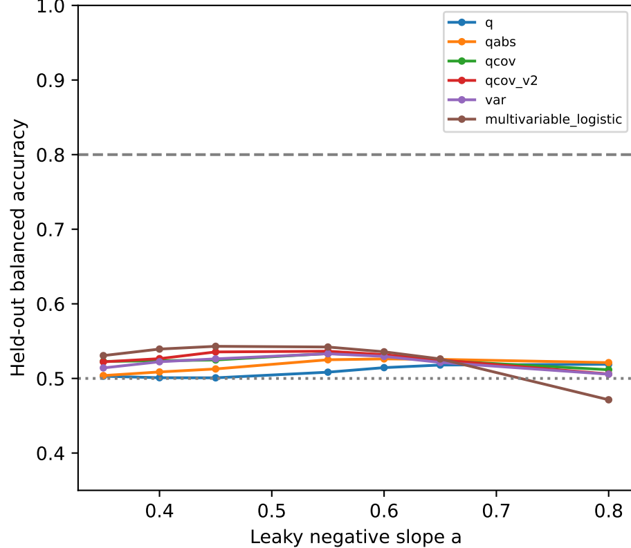
condA: next-task width contraction
