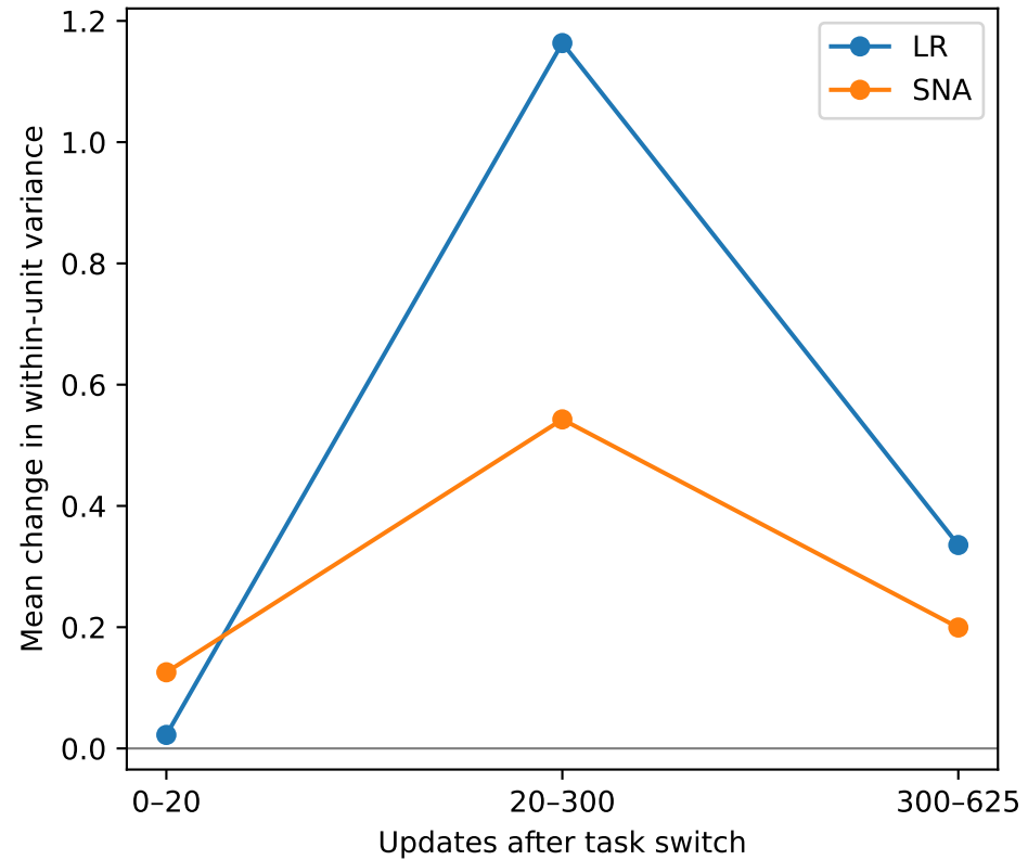
PM / Adam: variance change per phase
