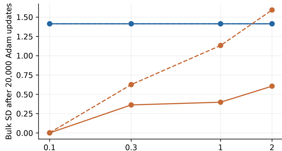
Initial bulk center b = -12
