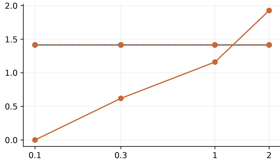
Initial bulk center b = -24
