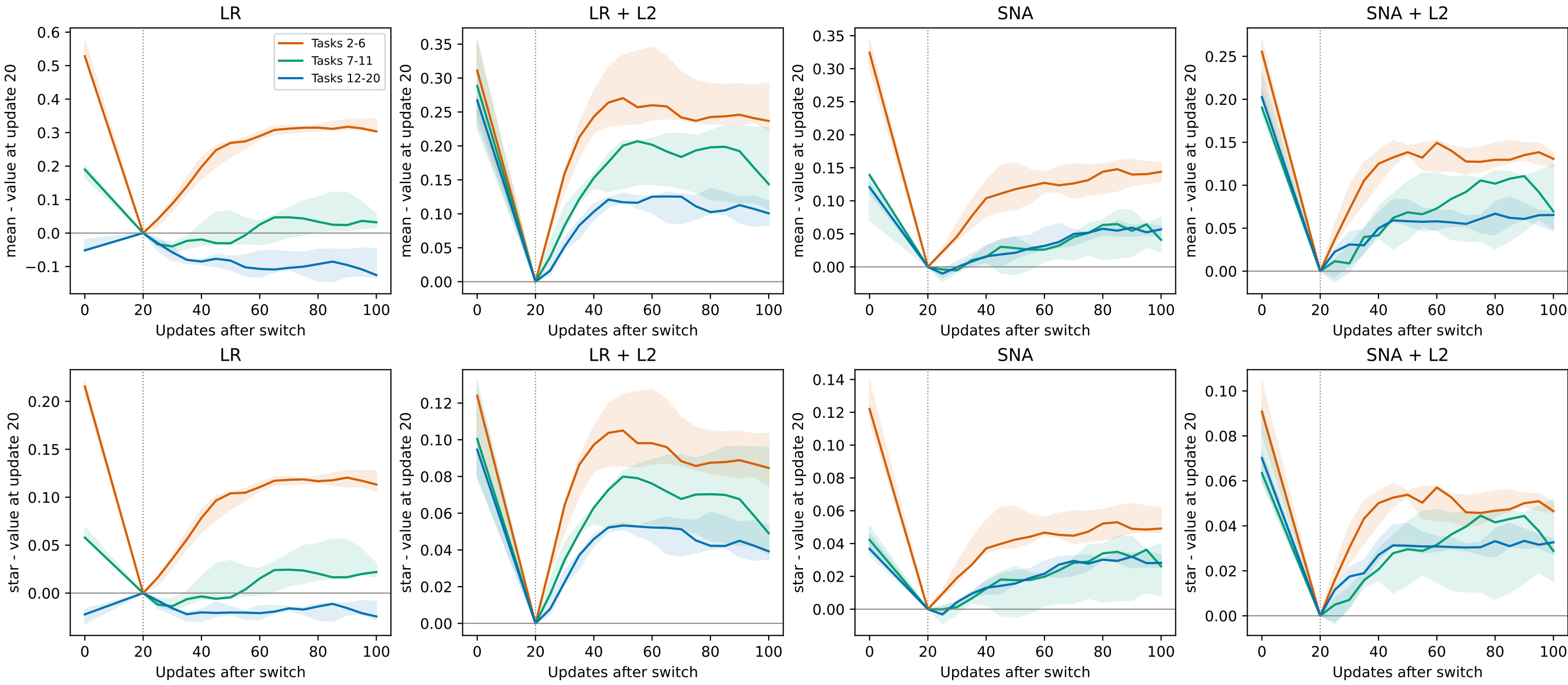
Does descent occur between updates 20 and 100? Same fixed inputs within each task; each line: seed median of task-bin means, shade: seed range
