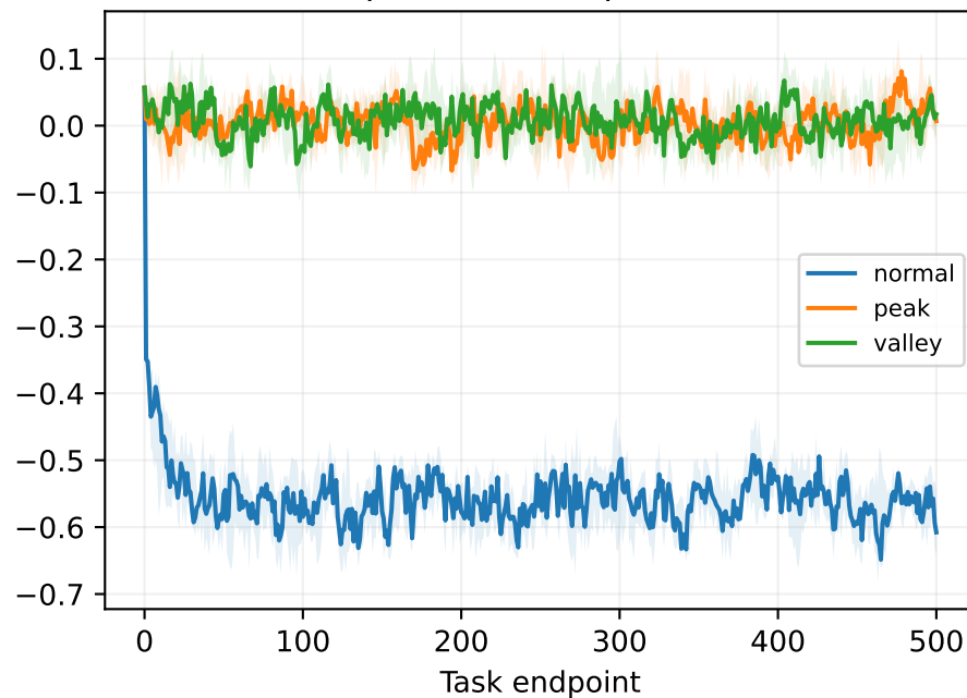
Leaky a=.1 offsets: free-weight RMS
