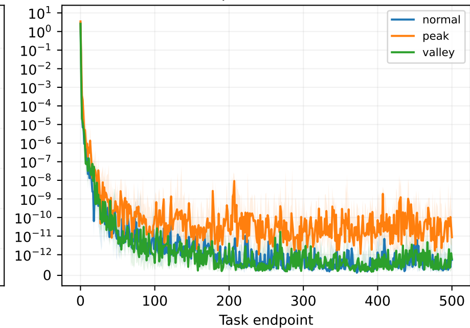
Full incoming-weight RMS
