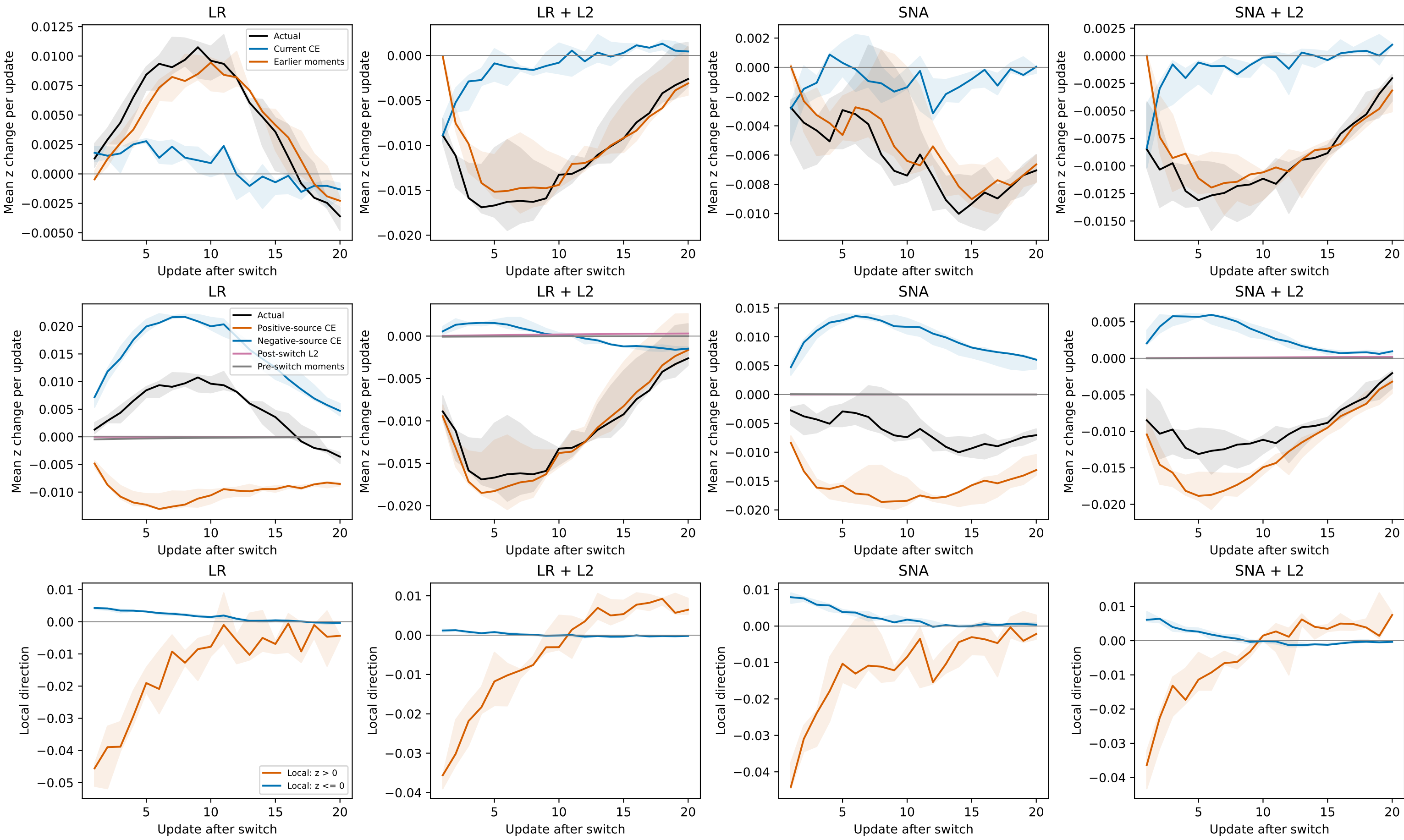
Task21..40: first update and evolving gradient contributions Median and range of 3 seed means; local derivative and actual shared update are different quantities
