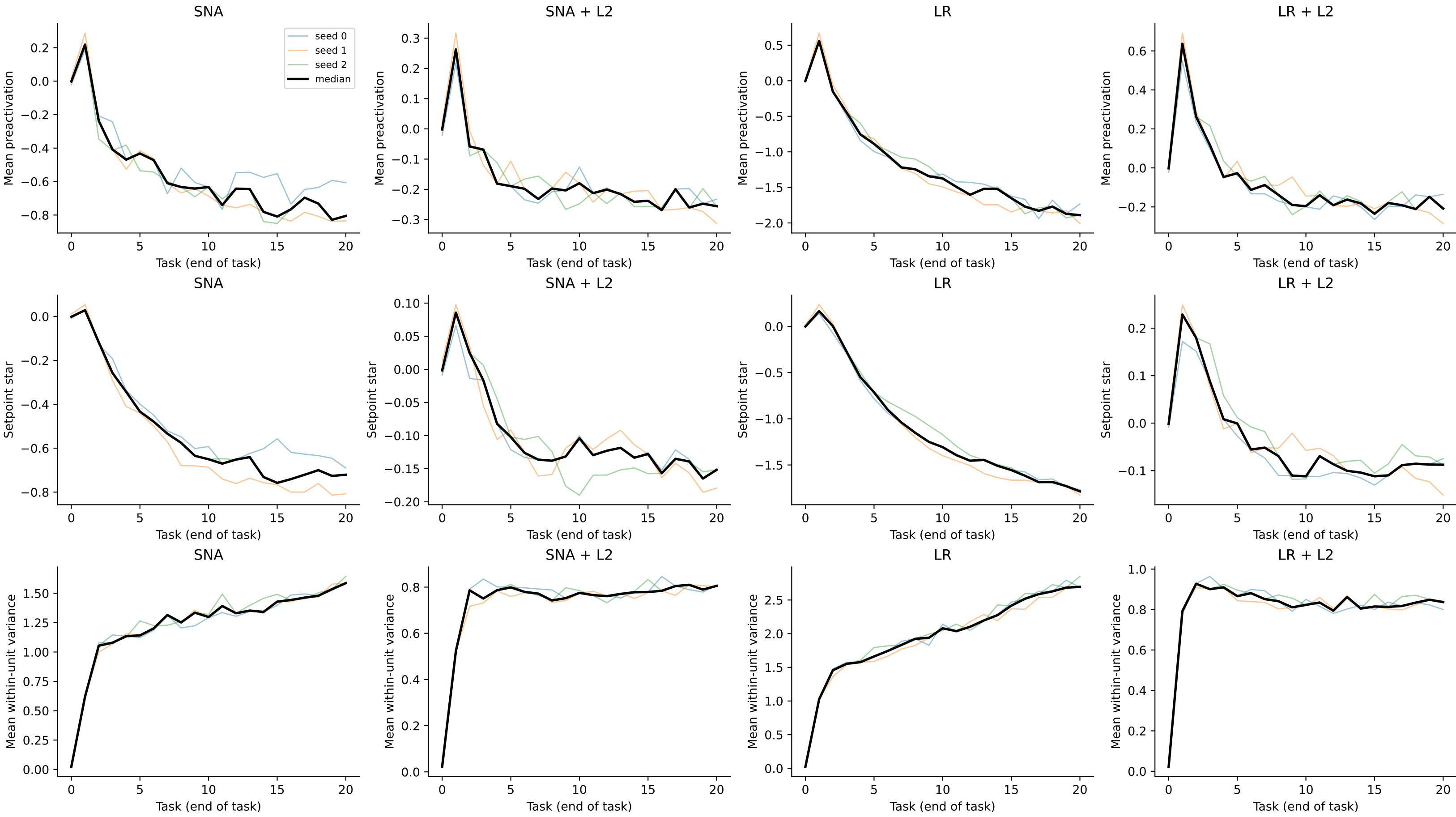
Formation from initialization through task 20 Task 0 = initialized parameters on task-1 inputs; tasks 1..20 = task end; same 3 seeds as late-window audit
