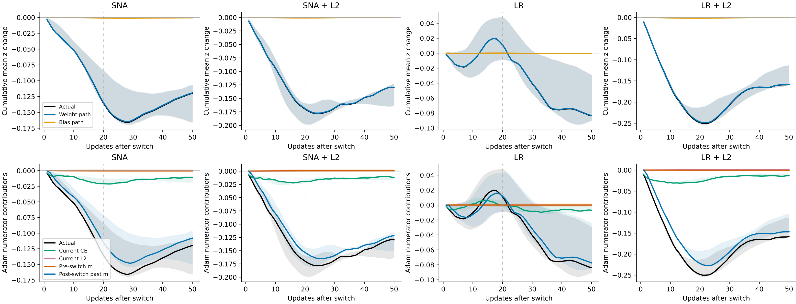
Early descent: parameter paths and Adam contributions CPU replay; 19 boundaries per seed; median and range of 3 seeds; step 0 = after permutation
