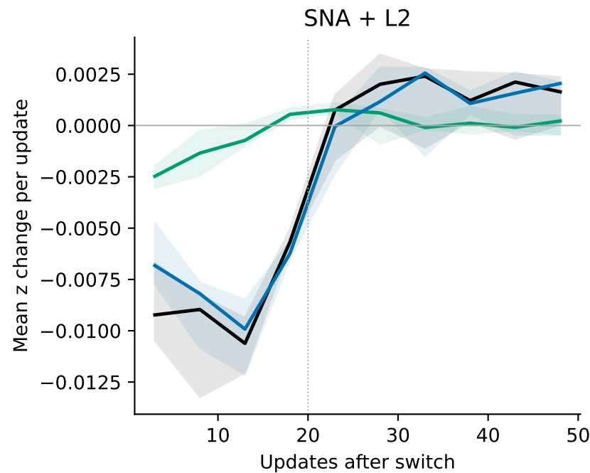
The gradient can turn upward before motion does Posthoc five-step averages; same actual Adam denominator for all numerator contributions
