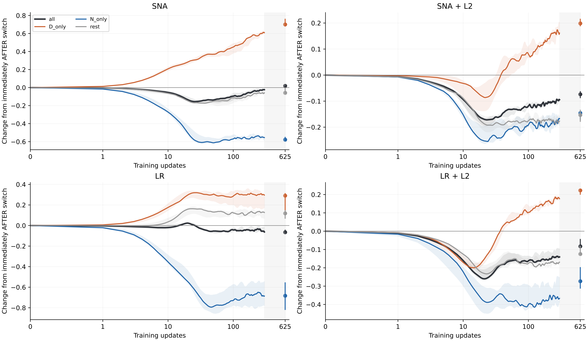
What LEARNING does after the instantaneous jump Original CUDA; per-seed average over tasks 101-119, then median and range of 3 seeds. Groups fixed at each boundary.
