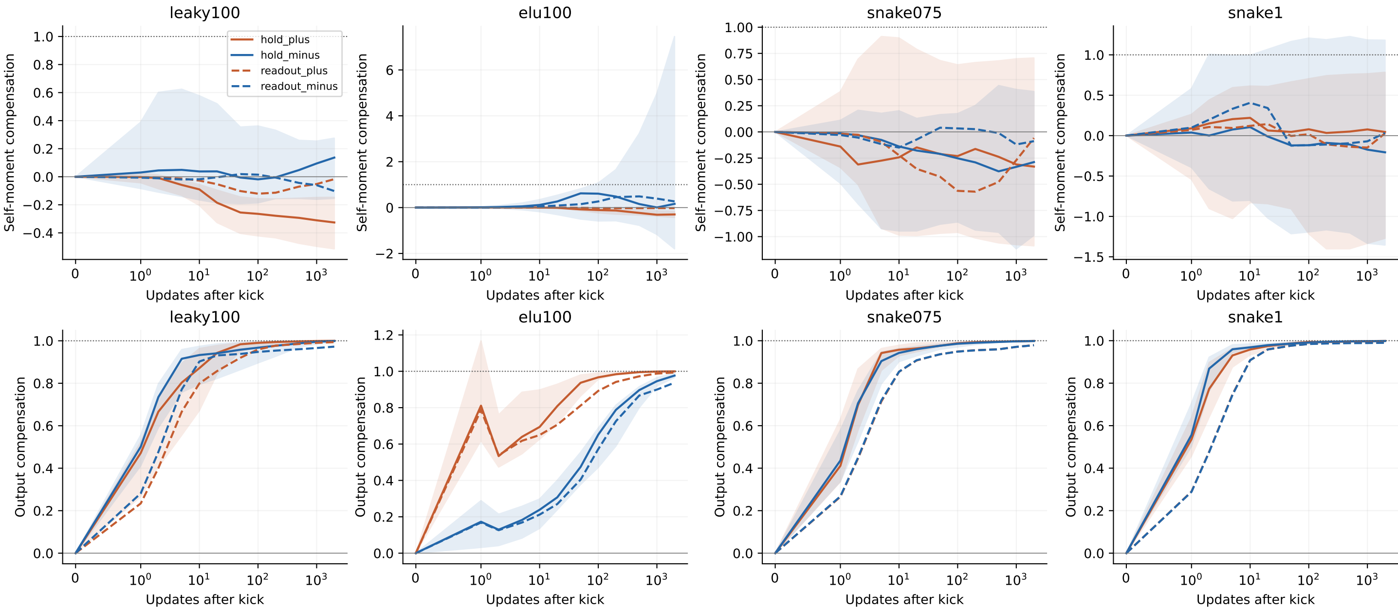
Pinned minority: do OTHER units compensate? Median and IQR across seeds Solid: other hidden units and readout learn. Dashed: readout only. Frozen task / full-batch GD.
