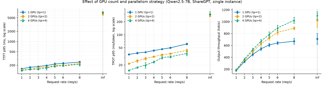
Figure 9. TTFT p95, TPOT p95 and output throughput against arrival rate for one, two and four GPUs (7B, ShareGPT). All three series were measured on one 4\times A40 instance, so host differences cannot contribute. Every tensor-parallel figure in this section was obtained with NCCL peer-to-peer transport and the custom all-reduce kernel disabled (§3.3); these are therefore conservative lower bounds on the achievable gain.
