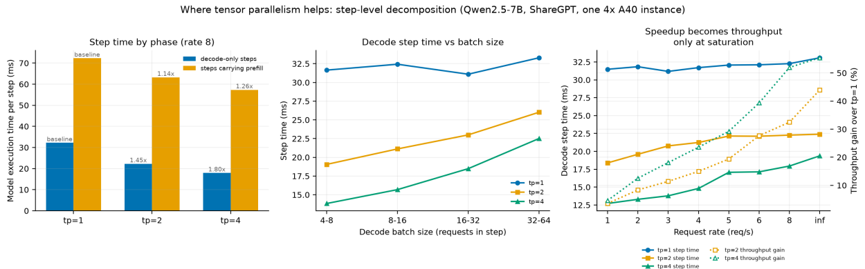
Figure 12. Why tensor parallelism helps, measured at step granularity (Qwen2.5-7B, ShareGPT,
