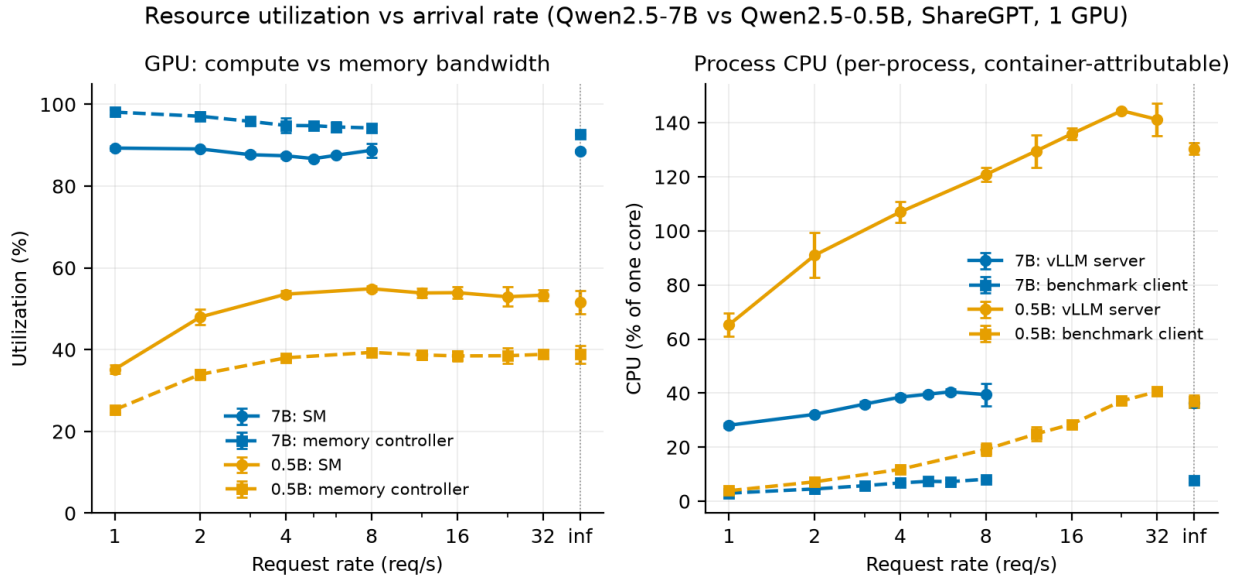
Figure 13. Resource utilization against arrival rate for the two model sizes (ShareGPT, one GPU). Left: GPU counters from pynvml — SM utilization is the fraction of time any kernel was resident, memory-controller utilization the fraction of time the controller was busy. The 7B curves sit near saturation on the memory controller while the 0.5B curves leave both counters below 60 %. Right: per-process CPU from psutil, in percent of a single core, so values above 100 % mean one process spanning more than one core. The two panels cross: moving from 7B to 0.5B lowers the GPU counters and raises the CPU curve. The models are swept over different rate grids ( \{1\ldots 8\} and \{1\ldots 32\} req/s, §3.3), so they overlap only up to rate 8. Samples are taken at 1 Hz and averaged over the measured section of each run, excluding start-up and warm-up (§3.4).
