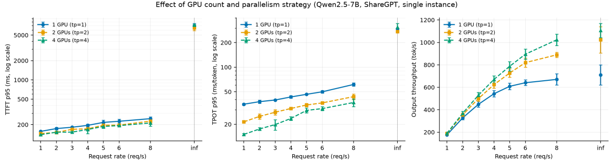
Figure 9. TTFT p95, TPOT p95 and output throughput against arrival rate for one, two and four GPUs (7B, ShareGPT). All three series were measured on one 4 \times A40 instance, so host differences cannot contribute. Every tensor-parallel figure in this section was obtained with NCCL peer-to-peer transport and the custom all-reduce kernel disabled (§3.3); these are therefore conservative lower bounds on the achievable gain.
