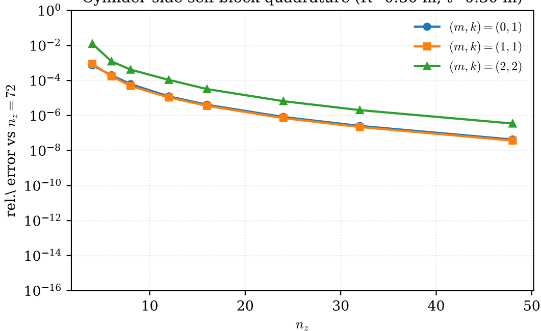
Cylinder-side self-block quadrature (R=0.30 m, t=0.30 m)
