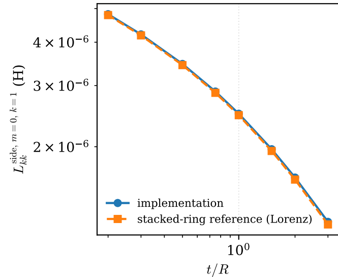
Short-solenoid self-inductance
