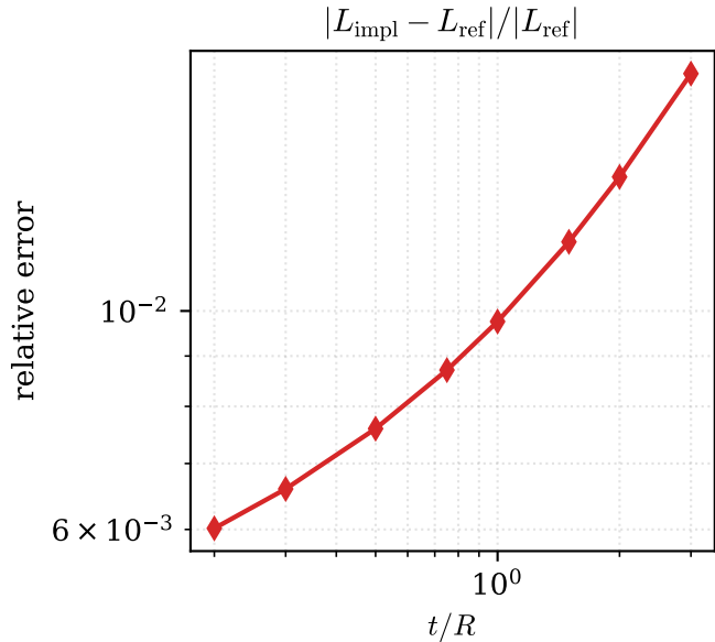
Short-solenoid self-inductance
