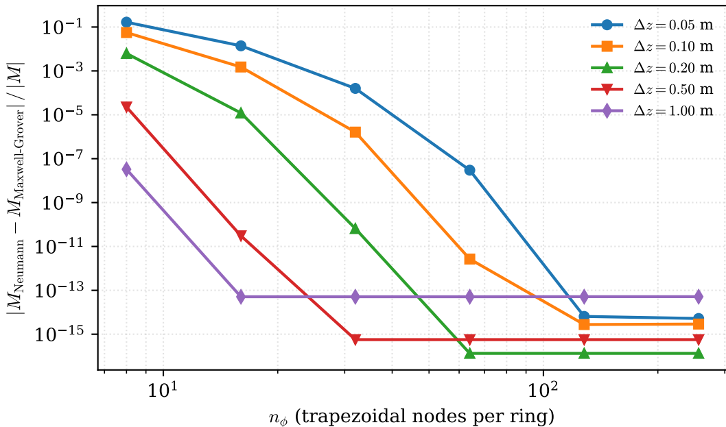
Coaxial-loop mutual: a = 0.30 m, b = 0.25 m
