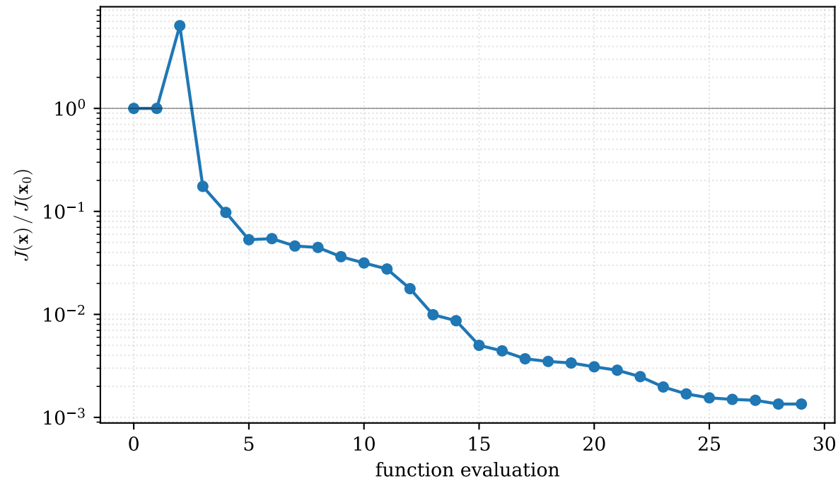
Coupled TF + passive-bulk optimization (L-BFGS-B)
