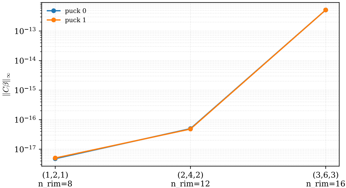
Rim continuity residual vs. basis resolution
