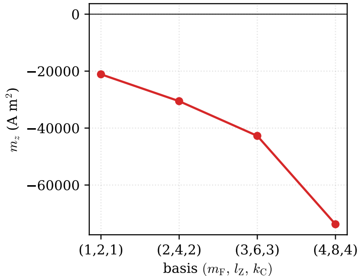
Lenz-sign check ( m_z < 0 expected)
