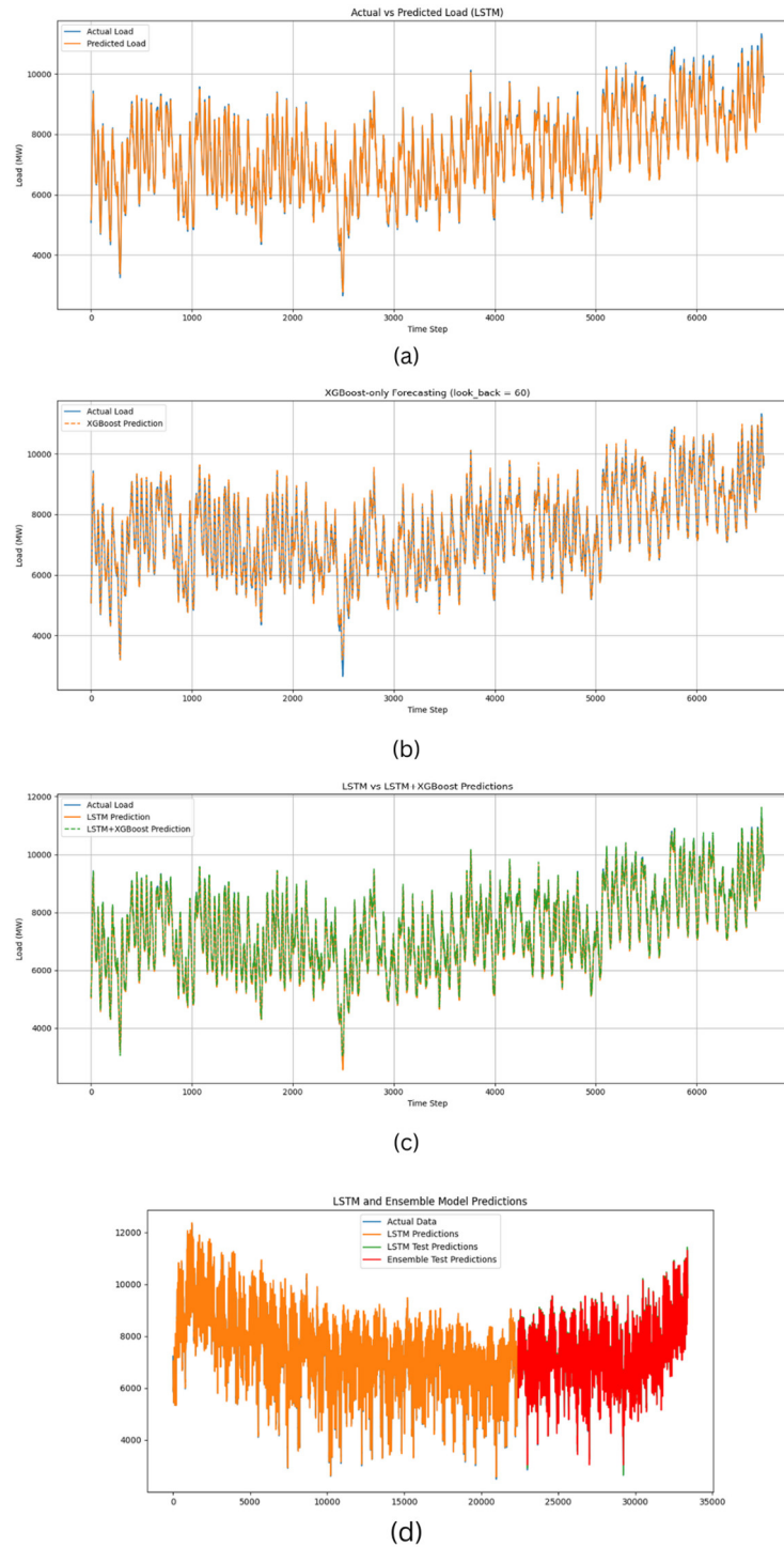
Figure 7. Visual comparison of actual electricity load with predictions generated by individual and hybrid models. (a) LSTM model predictions vs. actual load; (b) XGBoost model predictions vs. actual load; (c) Comparison of LSTM-only and LSTM+XGBoost hybrid model predictions against actual load; (d) Full-scale prediction including training and test results for both LSTM and ensemble model.
