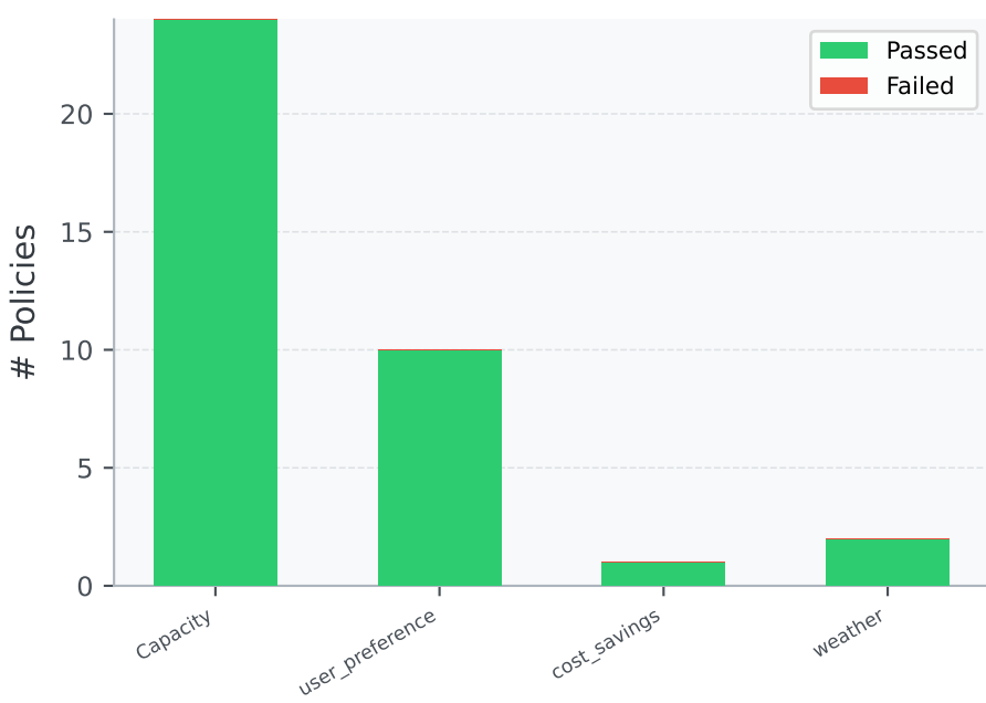
(f) Policies by Category
