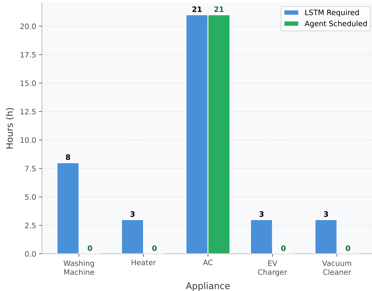
LSTM-Predicted vs Agent-Scheduled Runtime
