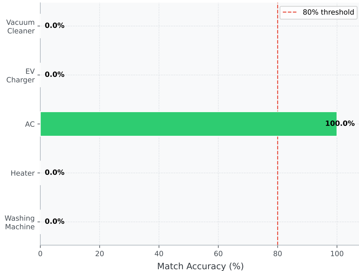
LSTM to Agent Schedule Match Accuracy (%)
