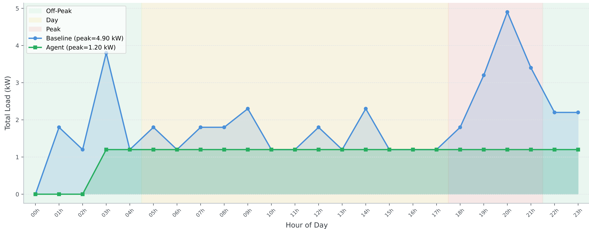
Hourly Aggregate Load Profile: Baseline vs. Optimised Agent
