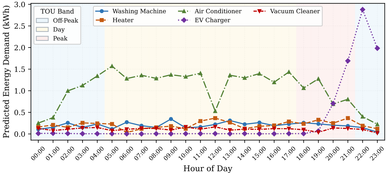
Fig. 2 -- LSTM-Predicted Hourly Energy Demand per Appliance (24 h)
