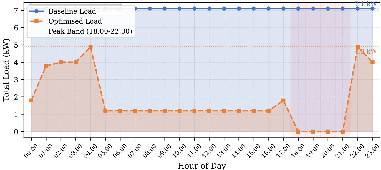
Fig. 4 -- 24-Hour Load Profile: Baseline vs. Optimised Agent
