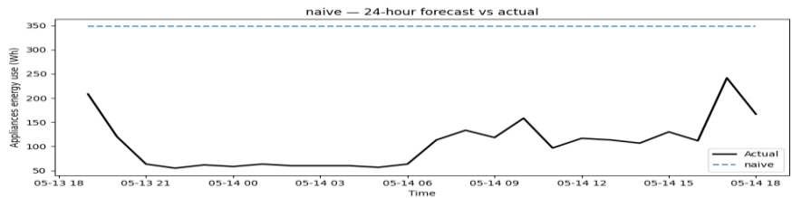
Figure A2. Naive forecast versus actual.
