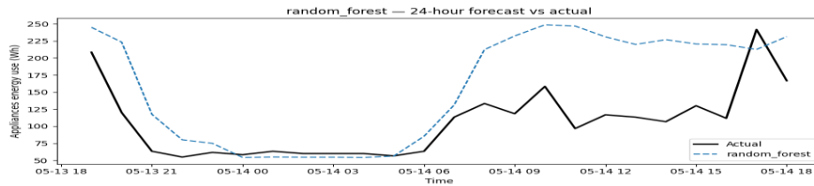
Figure A7. Random Forest forecast versus actual.
