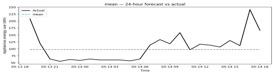
Figure A1. Mean forecast versus actual.
