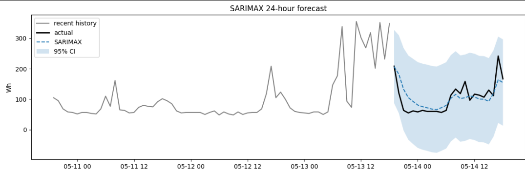
Figure 4. SARIMAX 24-hour forecast with 95% confidence interval.
