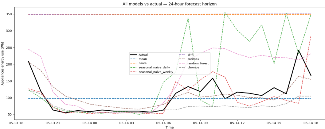
Figure 7. Forecast comparison across all models and actual observations.
