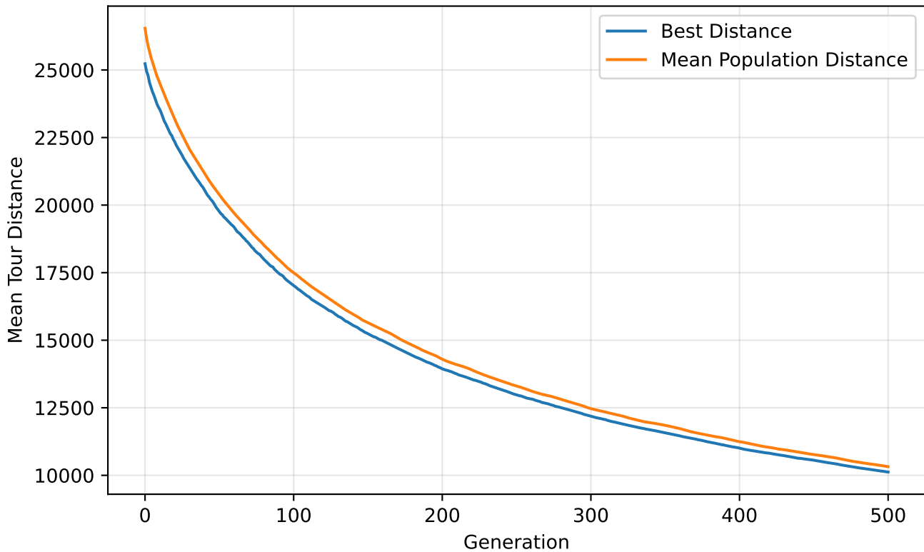
GA Convergence - 500 Cities
