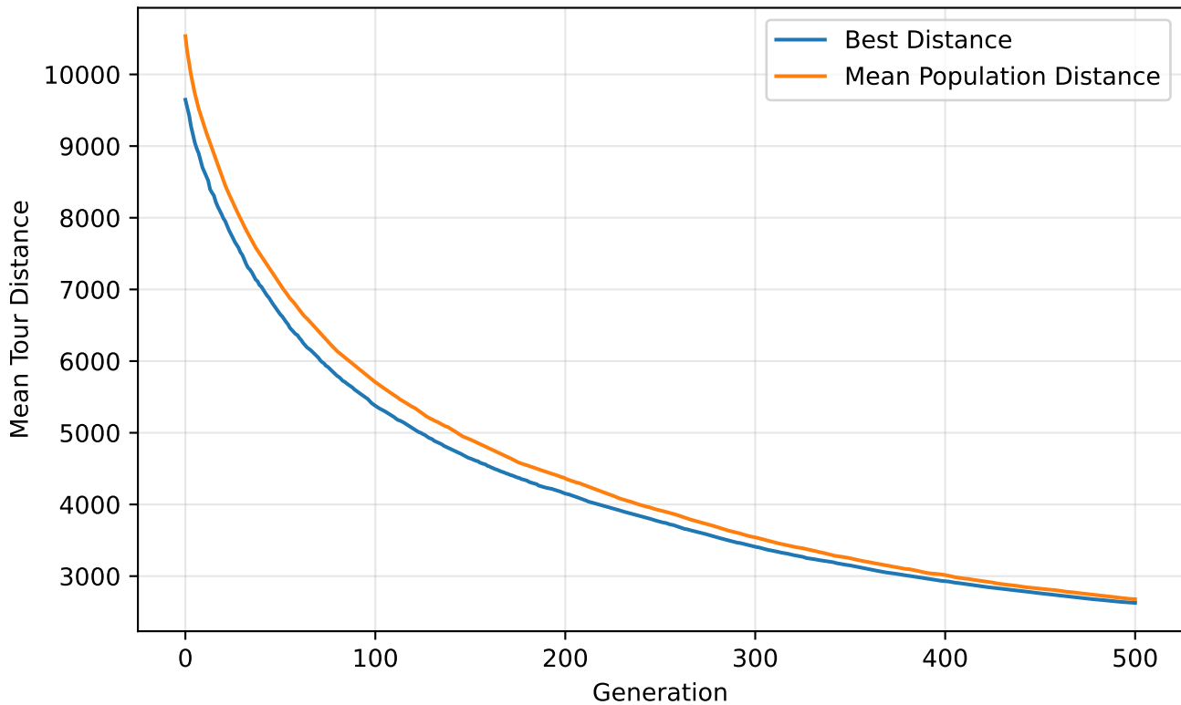
GA Convergence - 200 Cities
