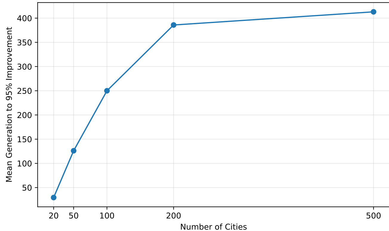
Convergence Speed vs Problem Size
