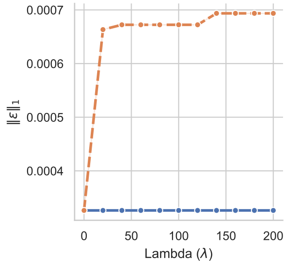
Candidate-level slack
