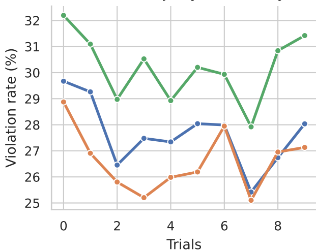
Pairwise Majority Consistency
