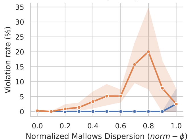
Pareto Optimality
