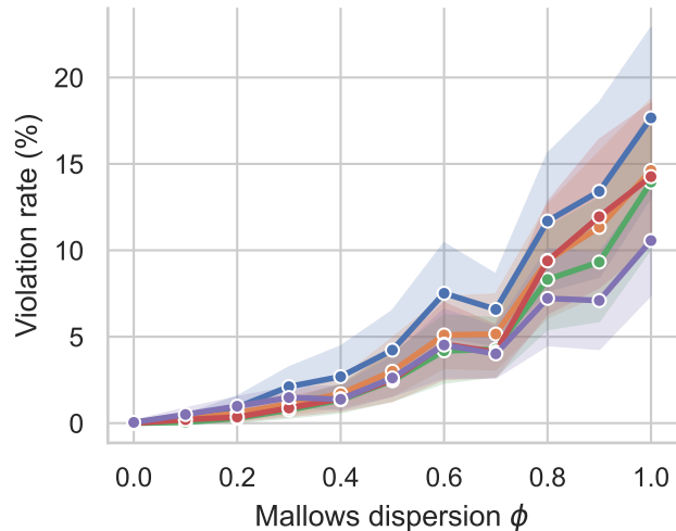
Pareto Optimality
