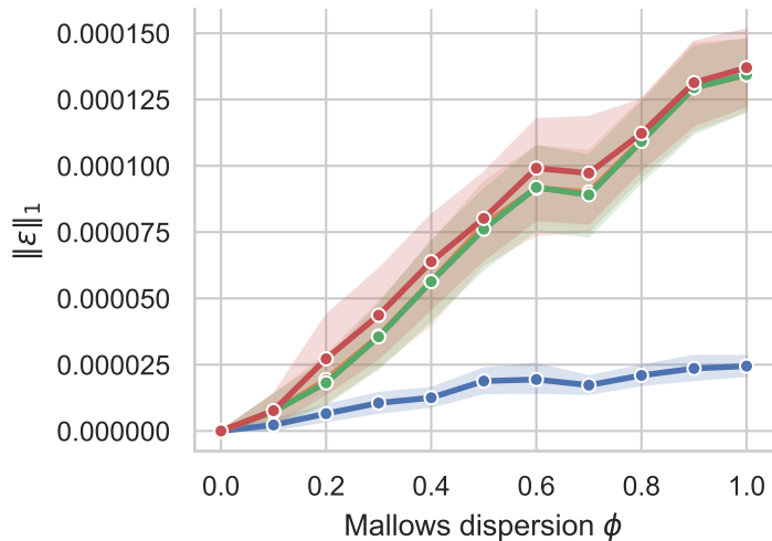
Candidate-level repair
