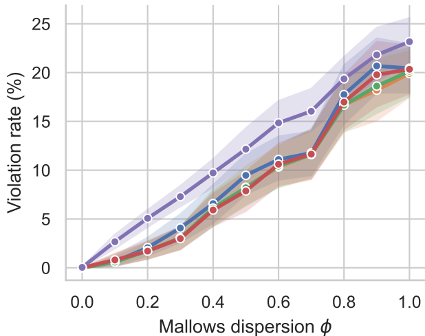
Total violations
