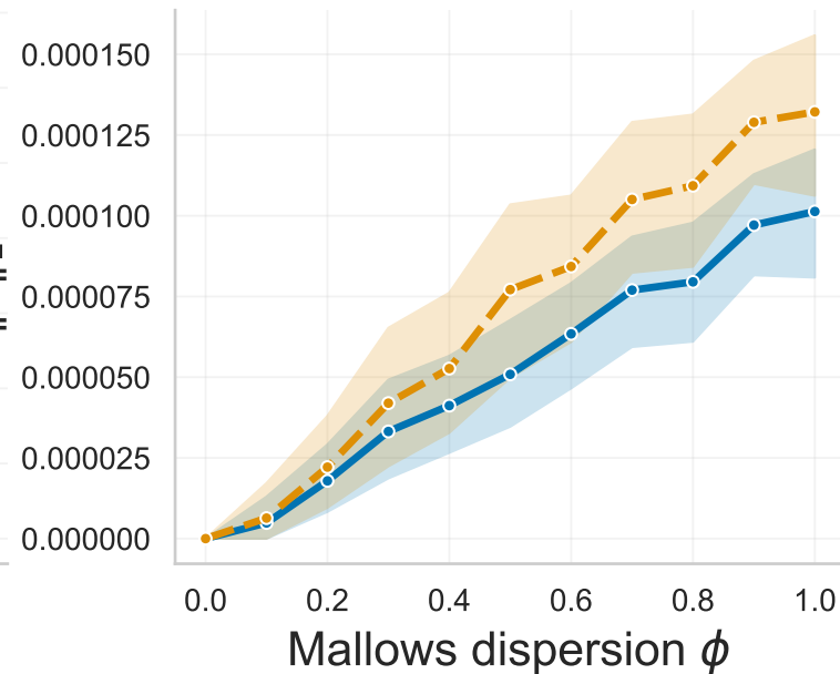
Candidate-wise slack
