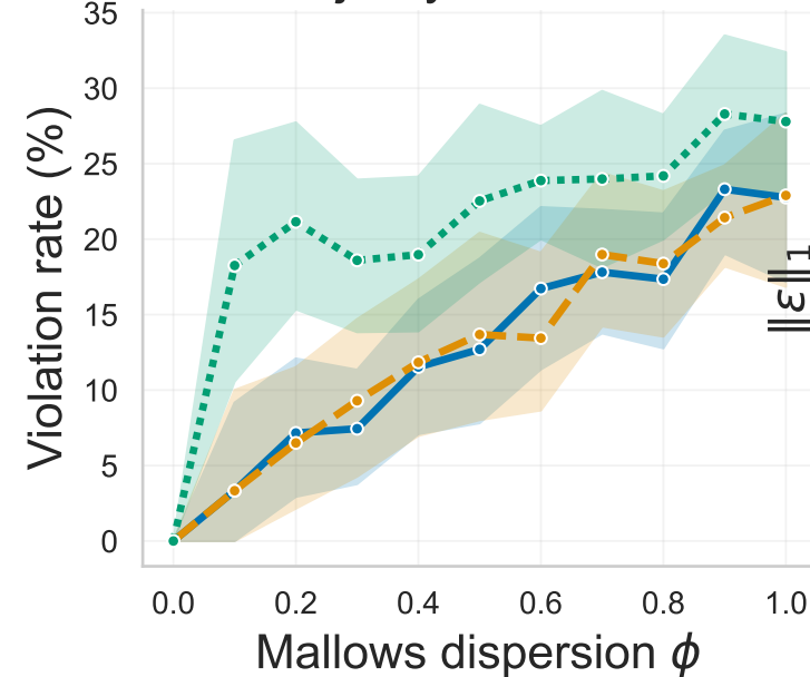
Majority Violations
