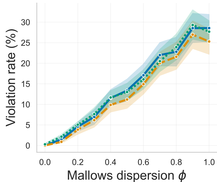
Total Violations
