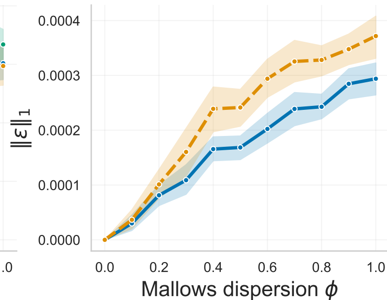
Candidate-wise slack
