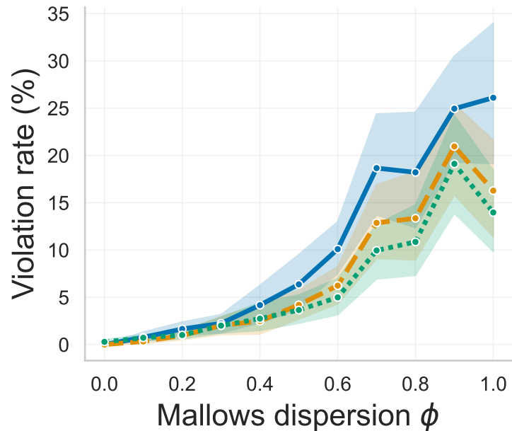
PO Violations
