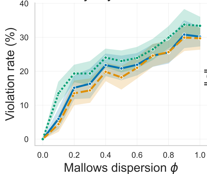
Majority Violations
