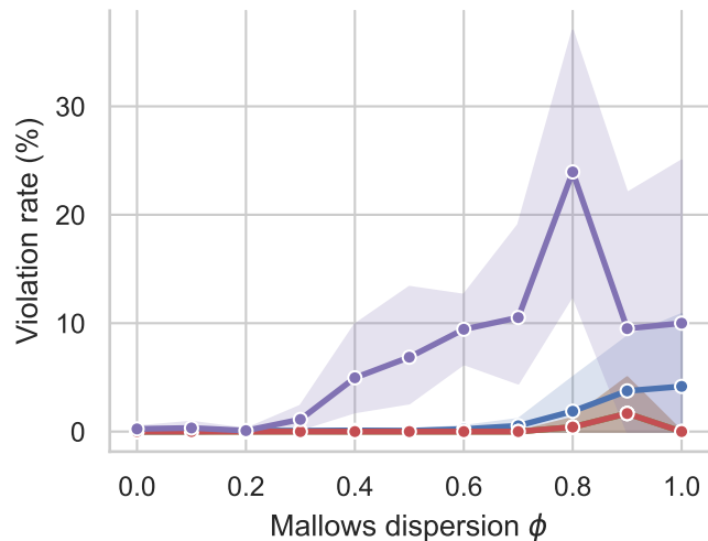
Pareto Optimality
