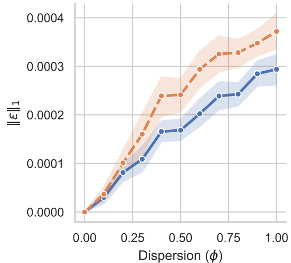
Candidate-level slack
