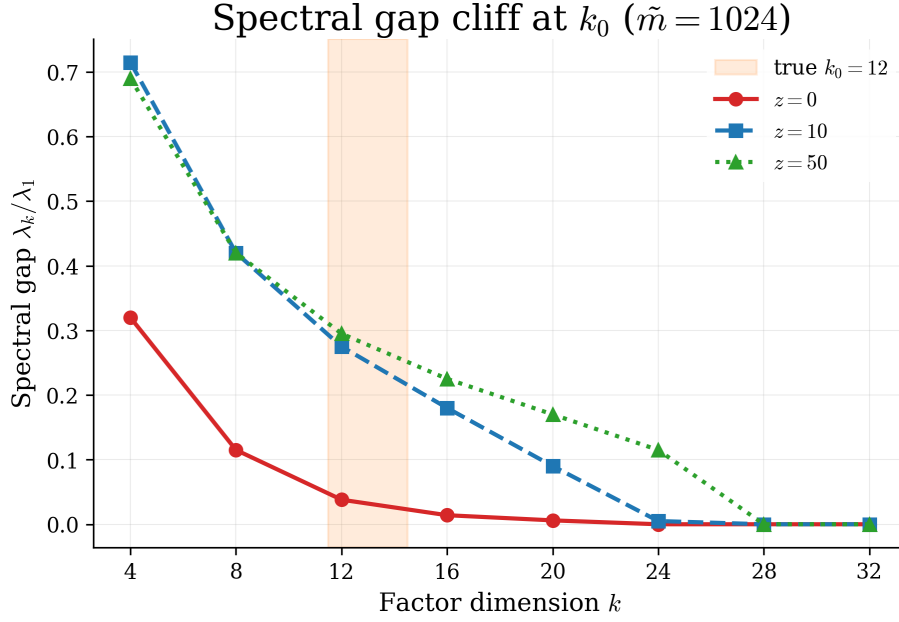
Figure 5: Spectral gap \lambda_k/\lambda_1 versus factor dimension k at \tilde{m} = 1024 for three ridge values z \in \{0, 10, 50\} . The shaded vertical band marks the true synthetic signal rank k_0 = 12 . The cliff at k_0 is sharp because the synthetic DGP has an exact rank cutoff; the regularized curves show the strongest gap, consistent with the ridge–curvature mechanism of Theorem 6.1(ii).
