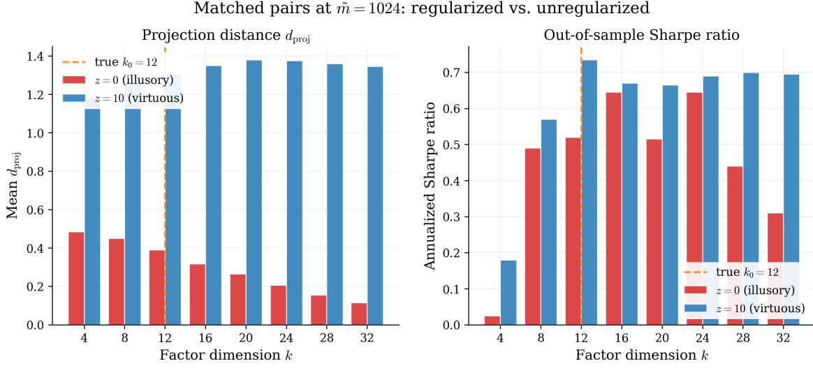
Figure 2: Matched pairs at \tilde{m} = 1024 : mean projection distance d_{\text{proj}} (left) and out-of-sample annualized Sharpe (right) at z = 0 (illusory) versus z = 10 (virtuous), as a function of the nominal factor dimension k . The orange dashed vertical line marks the true synthetic signal rank k_0 = 12 .
