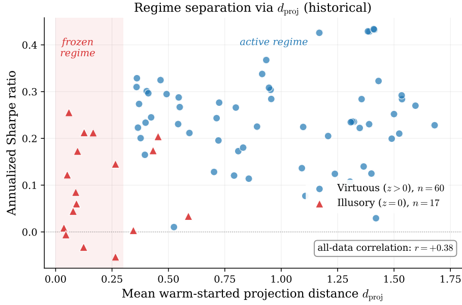
Figure 12: Annualized Sharpe ratio versus the mean warm-started projection distance d_{\text{proj}} across the historical configurations in our dataset. The shaded vertical region marks the frozen regime; unregularized configurations ( z = 0 , red triangles) cluster there, indicating warm-start solutions that barely move on the Grassmannian. Regularized configurations ( z > 0 , blue circles) move substantially farther from the warm start and occupy the active estimation regime. The all-data Pearson correlation between d_{\text{proj}} and Sharpe is reported in the inset.
