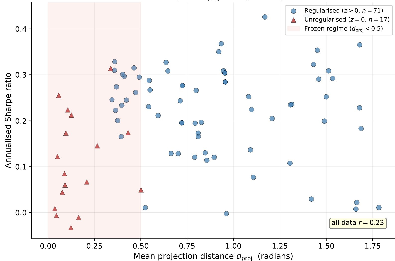
Historical: Sharpe vs d_{\text{proj}} — Regime Separation
