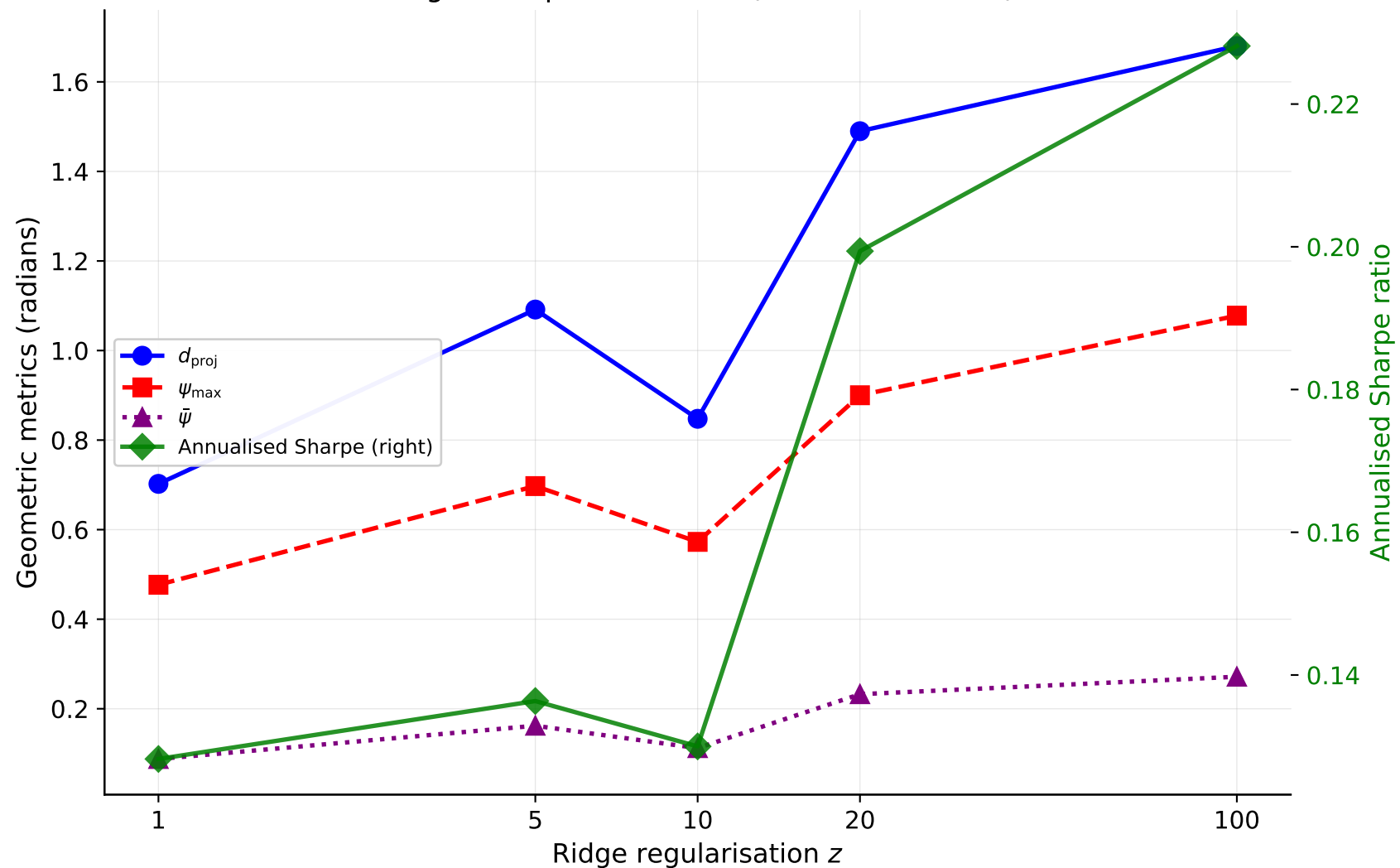
Ridge sweep — historical ( k = 12 , \tilde{m} = 1024 )
