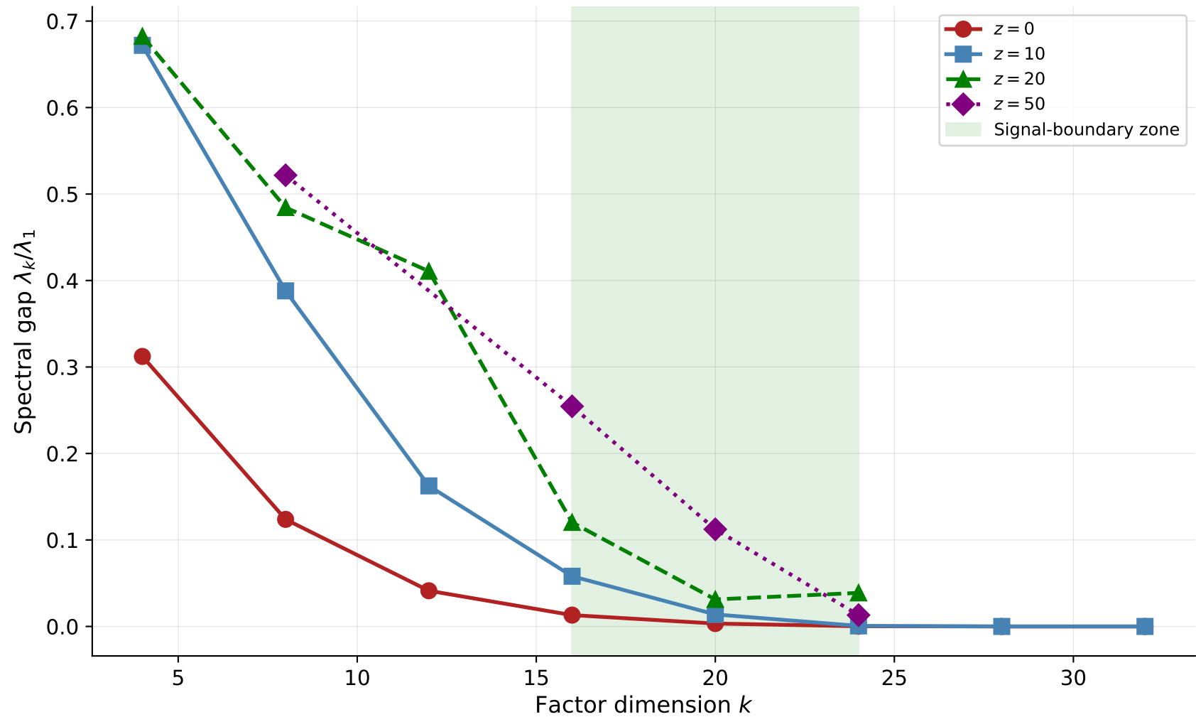
Spectral-gap cliff — historical ( \tilde{m} = 1024 )
