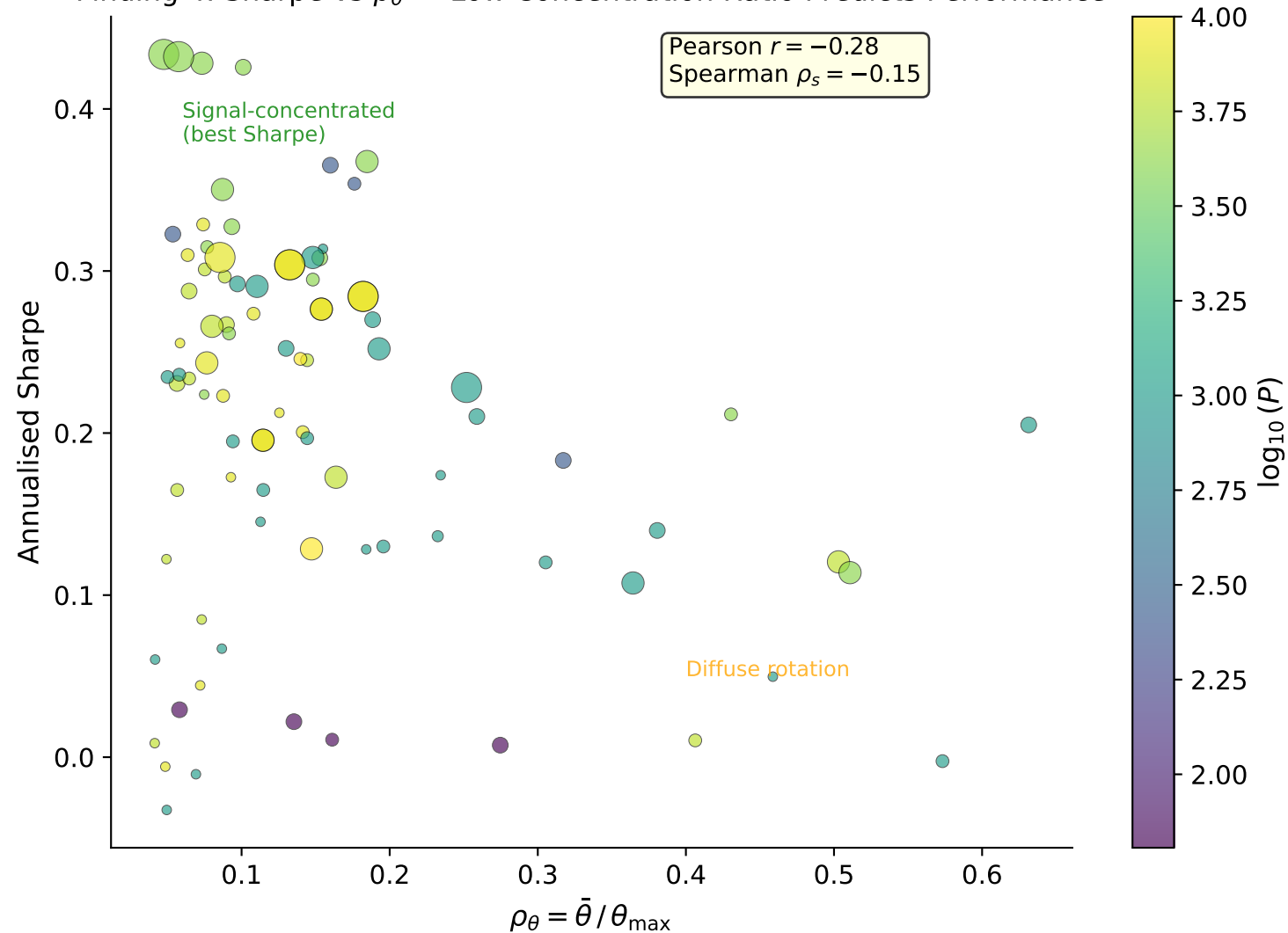
Finding 4: Sharpe vs \rho_\theta — Low Concentration Ratio Predicts Performance
